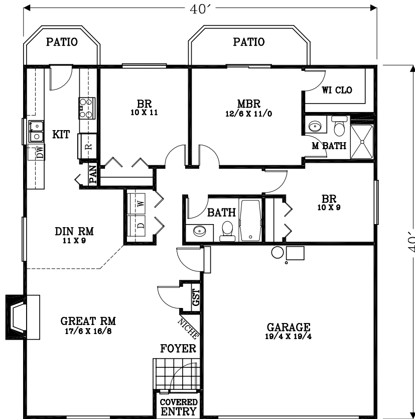
FLOOR PLAN 1192 SQUARE FEET
