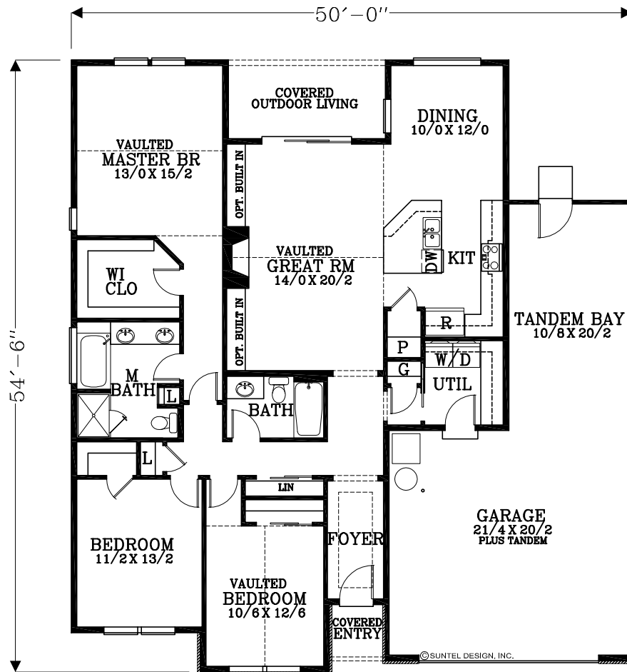
MAIN FLOOR PLAN 1707 SQUARE FEET
