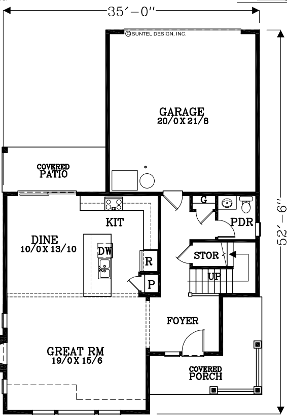
MAIN FLOOR PLAN 902 SQUARE FEET 2139 TOTAL SQUARE FEET
