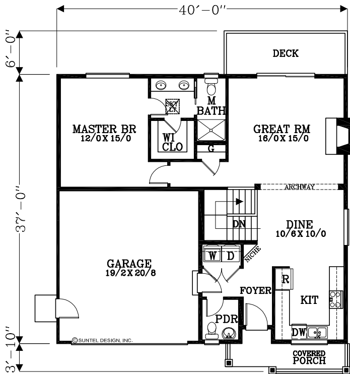
MAIN FLOOR PLAN 1050 SQUARE FEET 1765 TOTAL SQUARE FEET
