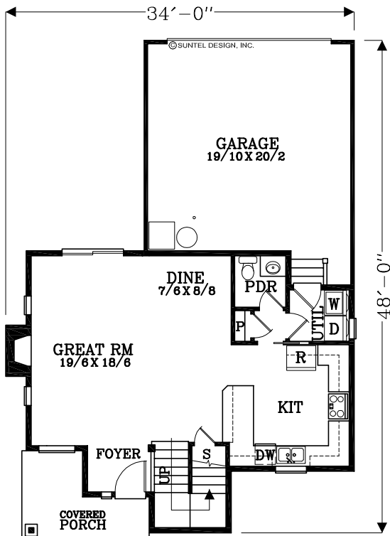
MAIN FLOOR PLAN 708 SQUARE FEET 1469 TOTAL SQUARE FEET
