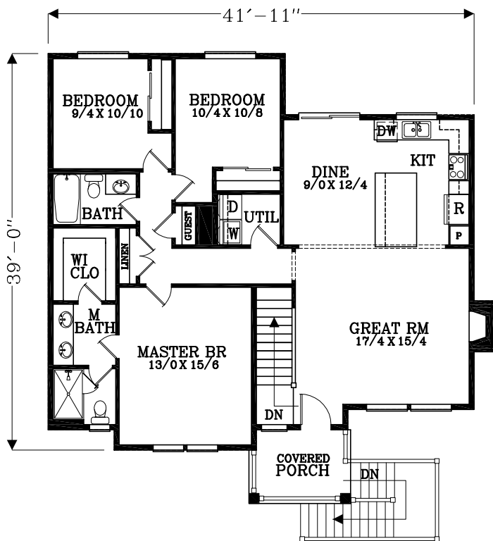
MAIN FLOOR PLAN 1442 SQUARE FEET
