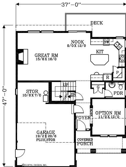
MAIN FLOOR PLAN 951 SQUARE FEET 2814 TOTAL SQUARE FEET
