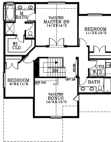
UPPER FLOOR PLAN 1187 SQUARE FEET
