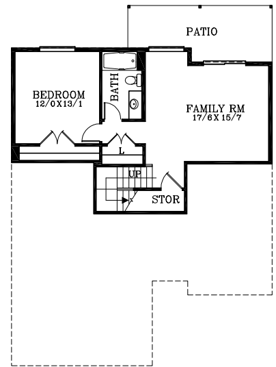
LOWER FLOOR PLAN 676 SQUARE FEET
