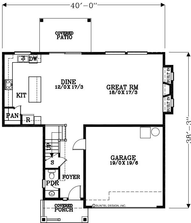
MAIN FLOOR PLAN 919 SQUARE FEET 2110 TOTAL SQUARE FEET
