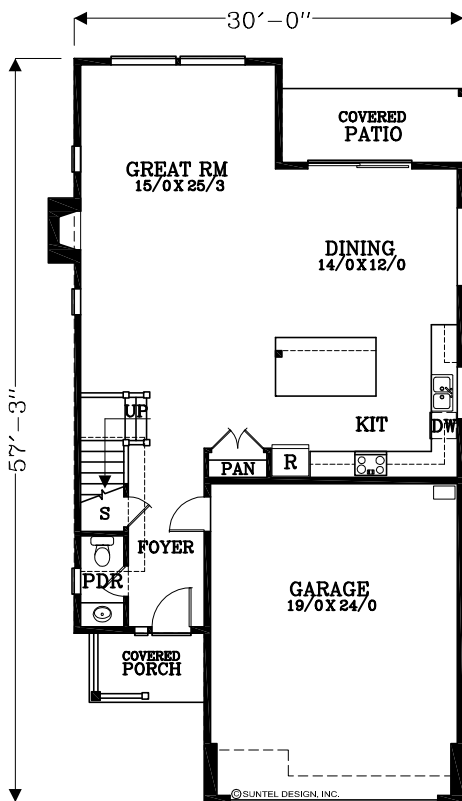
MAIN FLOOR PLAN 991 SQUARE FEET 2357 TOTAL SQUARE FEET
