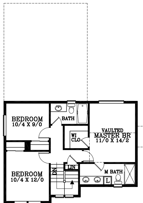
UPPER FLOOR PLAN 659 SQUARE FEET
