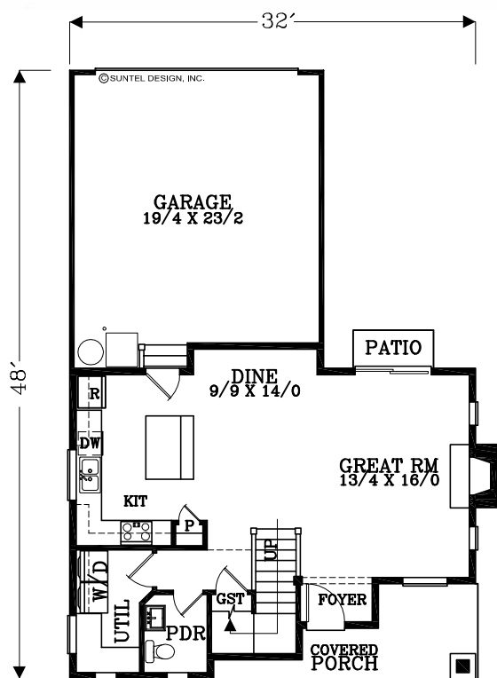
MAIN FLOOR PLAN 702 SQUARE FEET 1361 TOTAL SQUARE FEET
