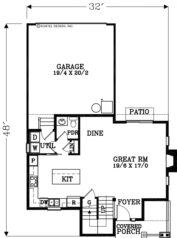
MAIN FLOOR PLAN 690 SQUARE FEET 1388 TOTAL SQ FT
