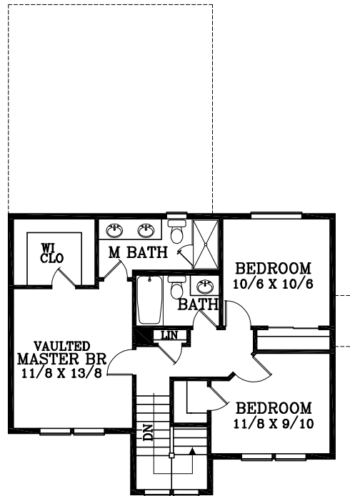
UPPER FLOOR PLAN 698 SQUARE FEET
