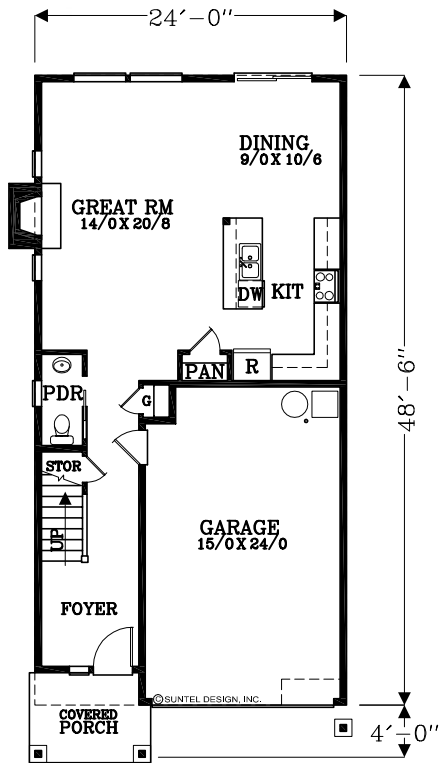
MAIN FLOOR PLAN 770 SQUARE FEET 1884 TOTAL SQUARE FEET
