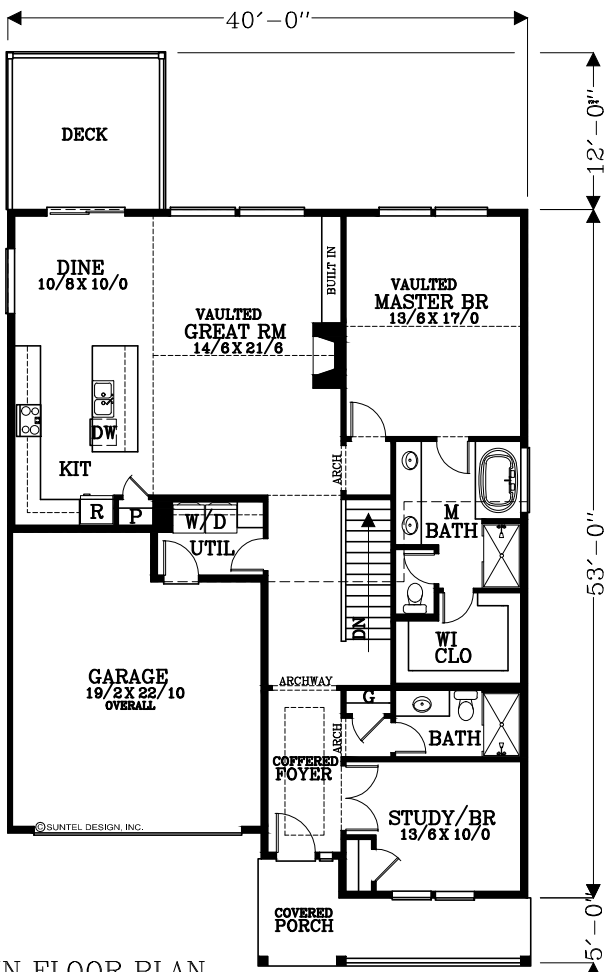
MAIN FLOOR PLAN 1585 SQUARE FEET 2559 TOTAL SQUARE FEET
