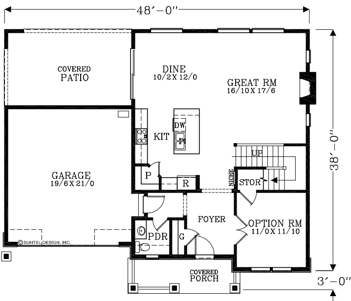
MAIN FLOOR PLAN 1024 SQUARE FEET 2629 TOTAL SQUARE FEET
