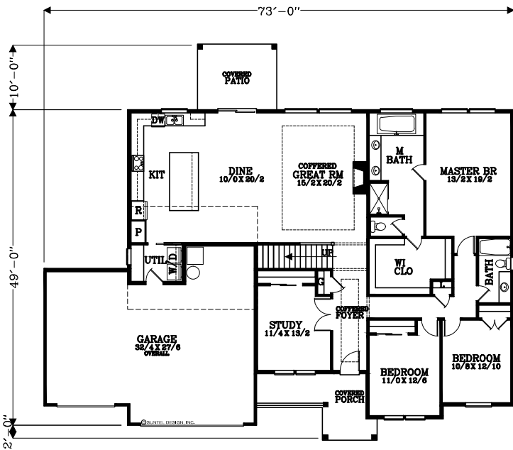
MAIN FLOOR PLAN 2263 SQUARE FEET 2585 TOTAL SQUARE FEET
