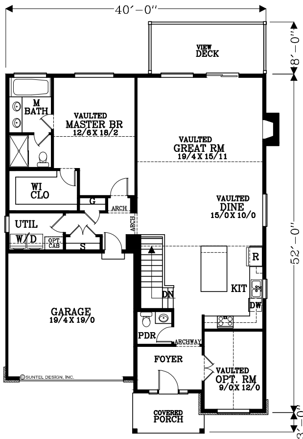
MAIN FLOOR PLAN 1567 SQUARE FEET 2579 TOTAL SQUARE FEET
