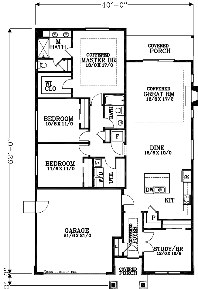
FLOOR PLAN 1870 SQUARE FEET
