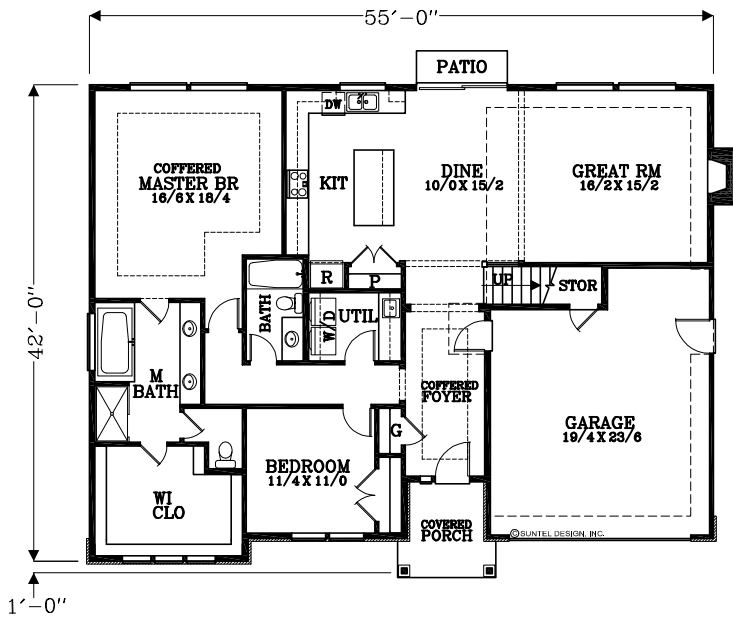
MAIN FLOOR PLAN 1760 SQUARE FEET 2382 TOTAL SQUARE FEET
