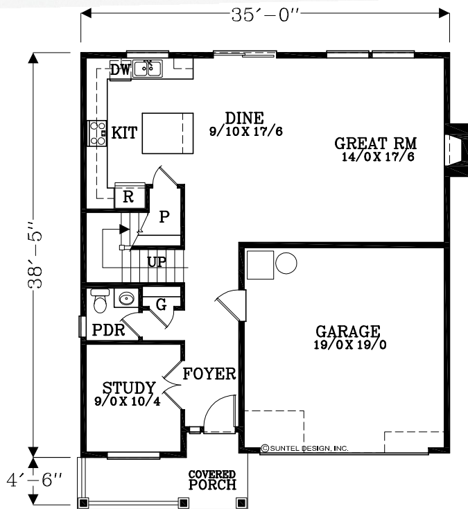
MAIN FLOOR PLAN 924 SQUARE FEET 2138 TOTAL SQUARE FEET
