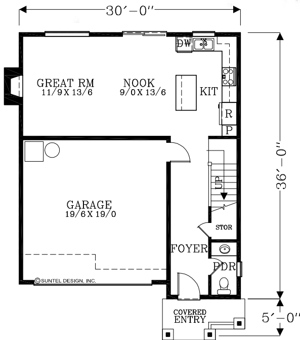
MAIN FLOOR PLAN 630 SQUARE FEET 1555 TOTAL SQUARE FEET
