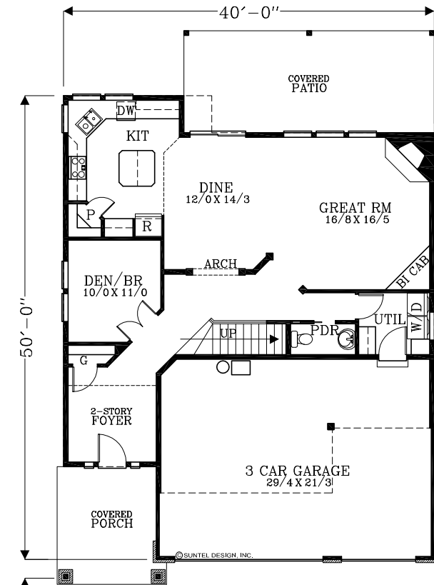
MAIN FLOOR PLAN 1132 SQUARE FEET 2517 TOTAL SQUARE FEET
