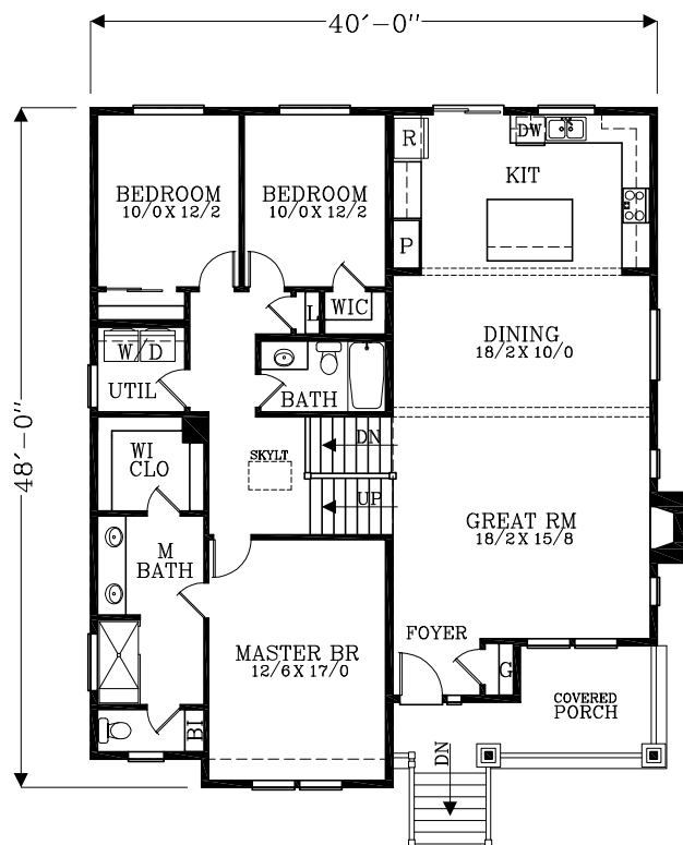
MAIN FLOOR PLAN 1,753 SQUARE FEET 2,231 TOTAL SQUARE FEET
