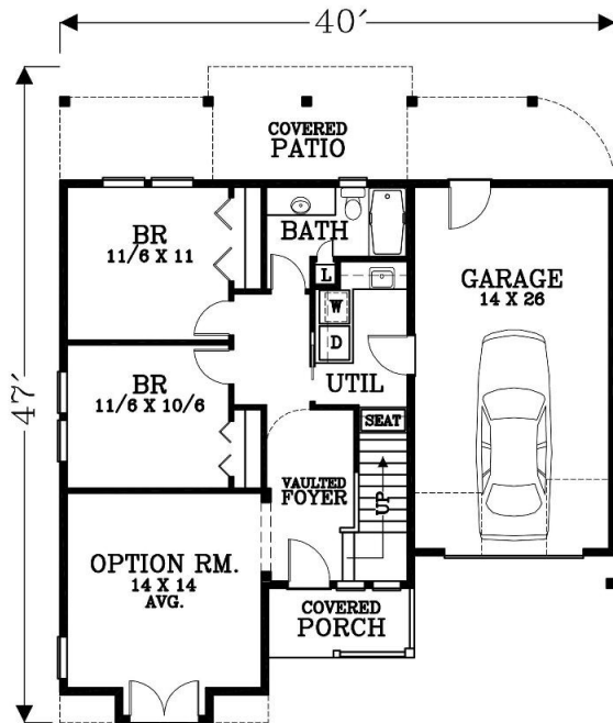
MAIN FLOOR PLAN 877 SQUARE FEET 2127 SQUARE FEET TOTAL
