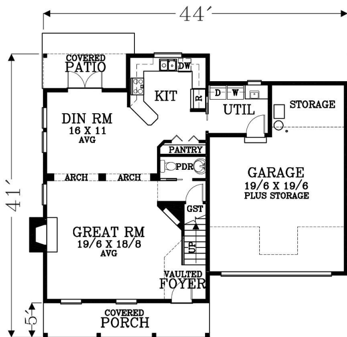
MAIN FLOOR PLAN 865 SQUARE FEET 1640 SQ FT TOTAL NIC BONUS
