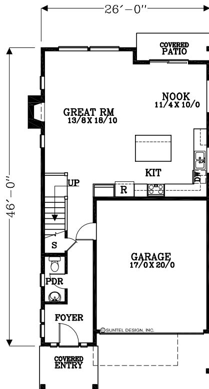
MAIN FLOOR PLAN 760 SQUARE FEET 1907 TOTAL SQUARE FEET
