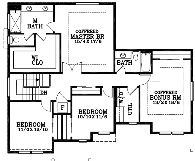
UPPER FLOOR PLAN 1384 SQUARE FEET
