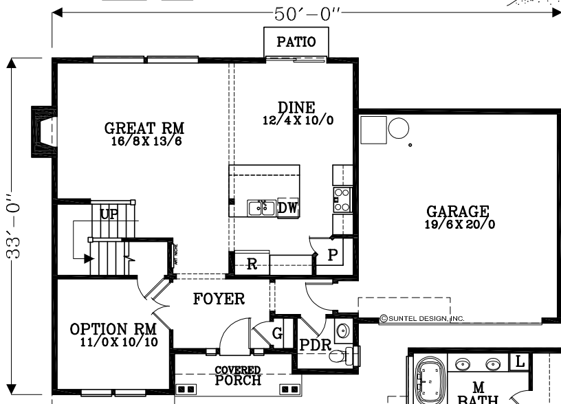
MAIN FLOOR PLAN 931 SQUARE FEET 2211 TOTAL SQUARE FEET
