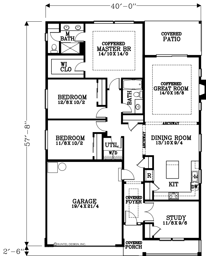
FLOOR PLAN 1,703 TOTAL SQUARE FEET
