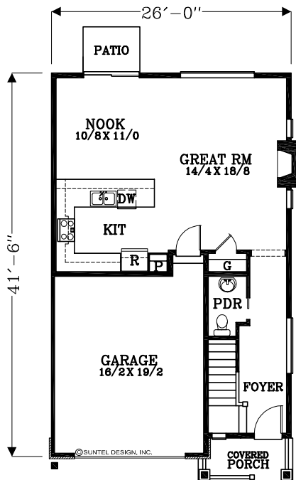
MAIN FLOOR PLAN 710 SQUARE FEET 1723 TOTAL SQUARE FEET
