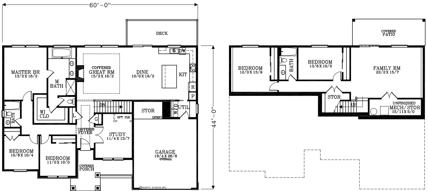
LOWER FLOOR PLAN 945 SQUARE FEET
