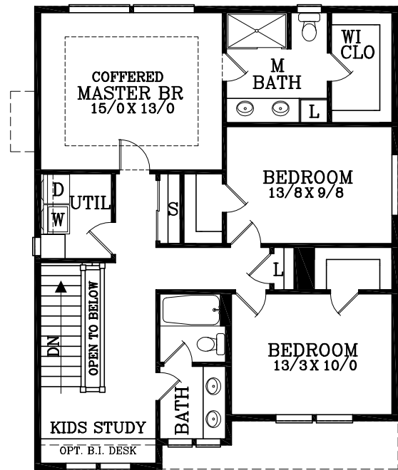
UPPER FLOOR PLAN 1025 SQUARE FEET
