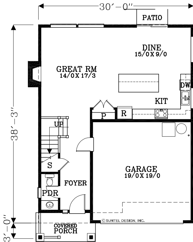
MAIN FLOOR PLAN 728 SQUARE FEET 1753 TOTAL SQUARE FEET
