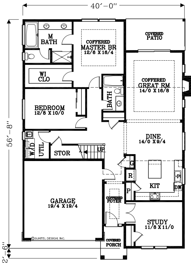
MAIN FLOOR PLAN 1700 SQUARE FEET 2383 TOTAL SQUARE FEET
