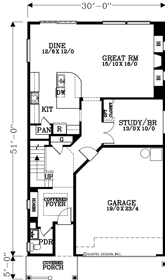
MAIN FLOOR PLAN 1054 SQUARE FEET 2428 TOTAL SQUARE FEET
