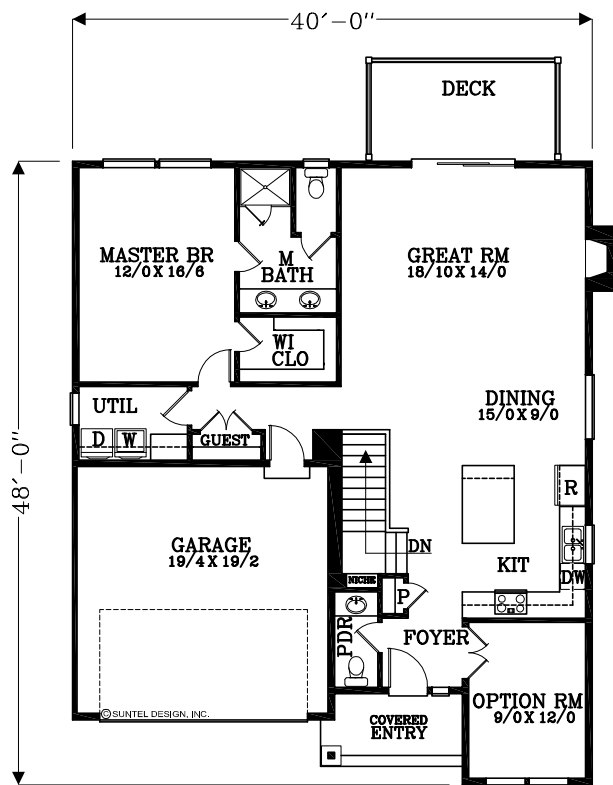
MAIN FLOOR PLAN 1,347 SQUARE FEET 2,192 TOTAL SQUARE FEET
