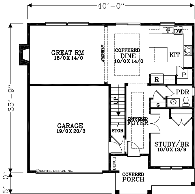
MAIN FLOOR PLAN 958 SQUARE FEET 2248 TOTAL SQUARE FEET
