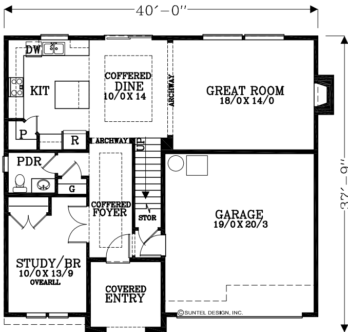
MAIN FLOOR PLAN 958 SQUARE FEET 2248 TOTAL SQUARE FEET
