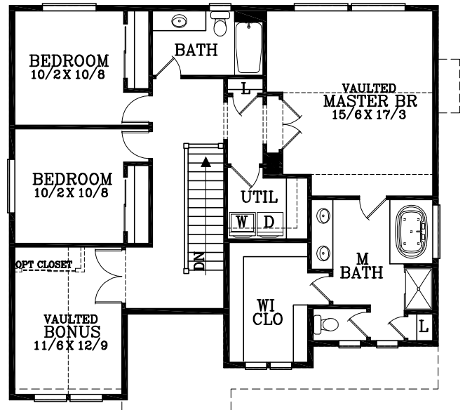
UPPER FLOOR PLAN 1290 SQUARE FEET
