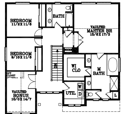
UPPER FLOOR PLAN 1359 SQUARE FEET
