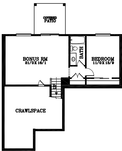
LOWER FLOOR PLAN 696 SQUARE FEET
