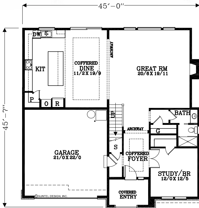
MAIN FLOOR PLAN 1380 SQUARE FEET 3154 TOTAL SQUARE FEET
