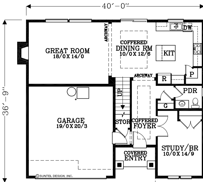
MAIN FLOOR PLAN 942 SQUARE FEET 2202 TOTAL SQUARE FEET
