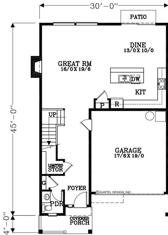
MAIN FLOOR PLAN 897 SQUARE FEET 2172 TOTAL SQUARE FEET
