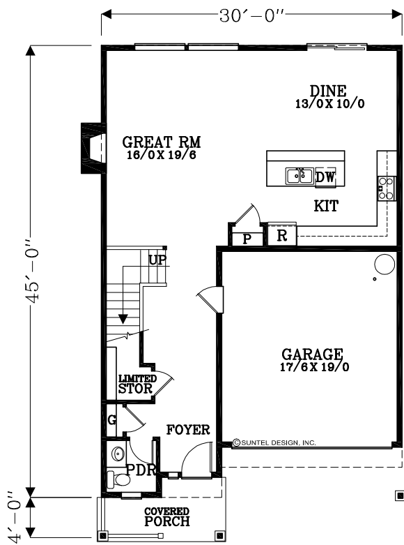
MAIN FLOOR PLAN 897 SQUARE FEET 2193 TOTAL SQUARE FEET
