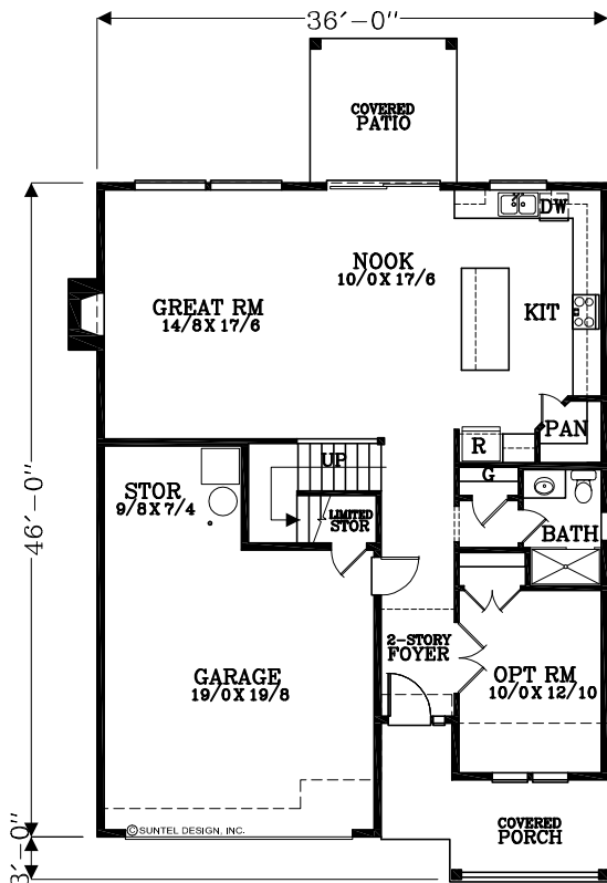
MAIN FLOOR PLAN 1100 SQUARE FEET 2466 TOTAL SQUARE FEET
