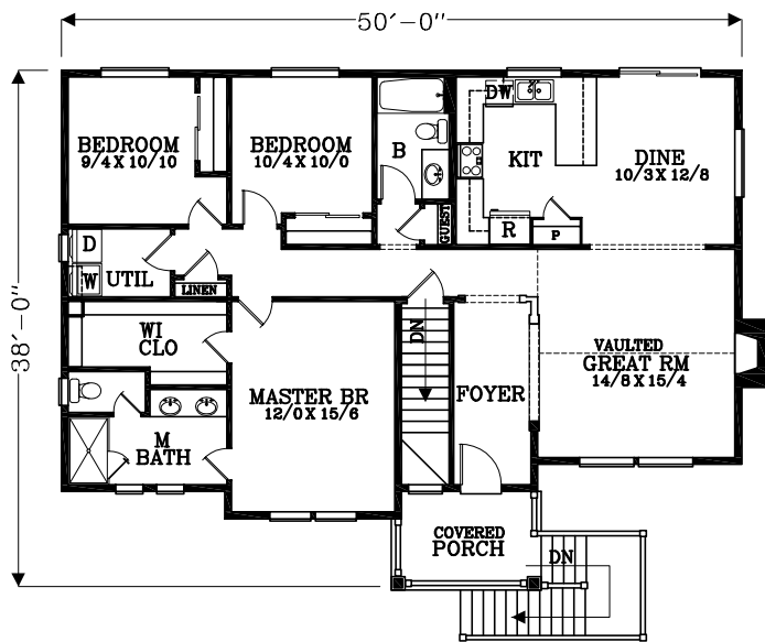
MAIN FLOOR PLAN 1546 SQUARE FEET
