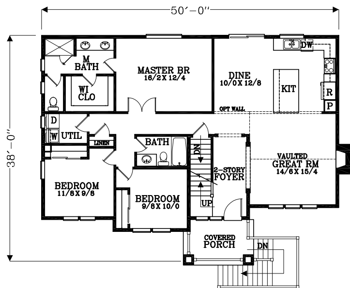
MAIN FLOOR PLAN 1546 SQUARE FEET 2099 TOTAL SQUARE FEET
