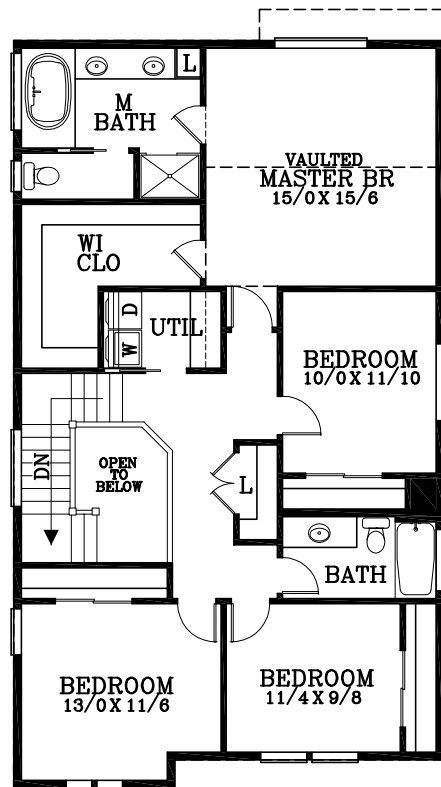
UPPER FLOOR PLAN 1213 SQUARE FEET
