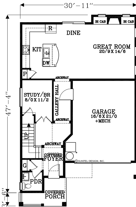
MAIN FLOOR PLAN 822 SQUARE FEET 2019 TOTAL SQUARE FEET
