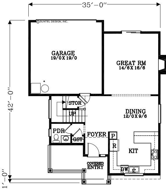
MAIN FLOOR PLAN 770 SQUARE FEET 1,843 TOTAL SQUARE FEET
