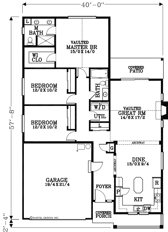
FLOOR PLAN 1544 TOTAL SQUARE FEET
