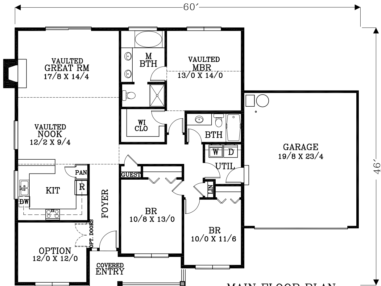
MAIN FLOOR PLAN 1683 TOTAL SQUARE FEET
