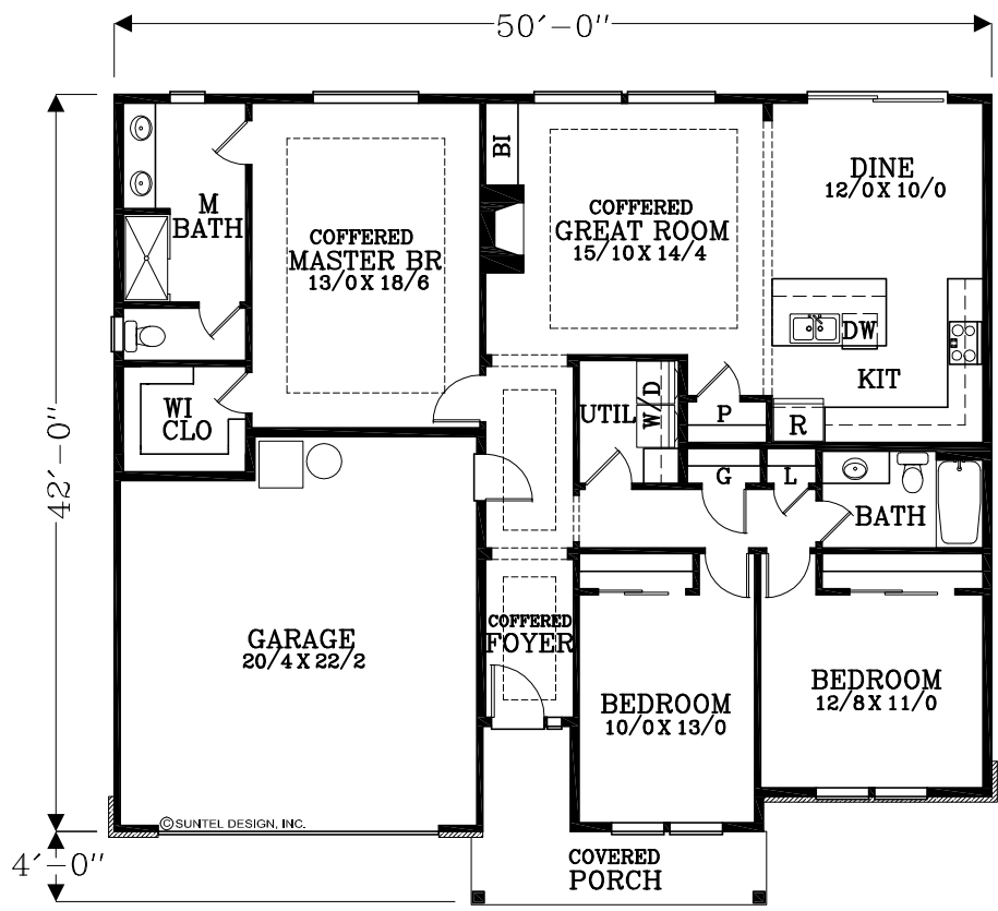
FLOOR PLAN 1577 TOTAL SQUARE FEET
